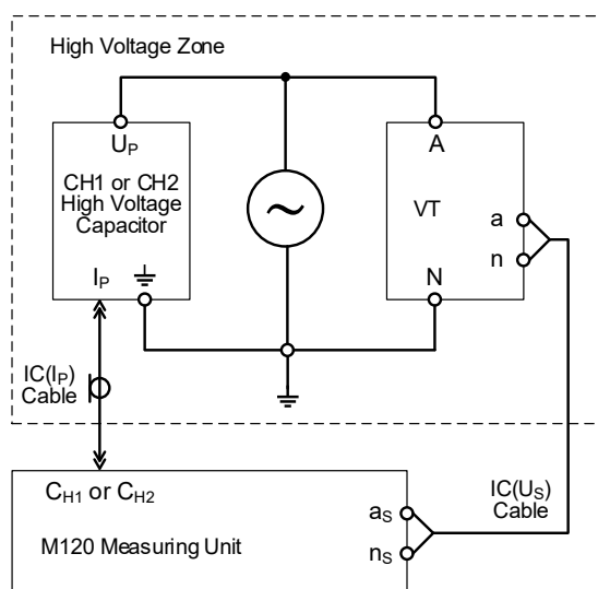
Fig. 1 Inductive VT, Capacitive VT testing
