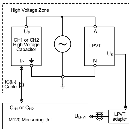
Fig. 2 Low-power VT (LPVT), Voltage sensor testing (for M120.2 only)
